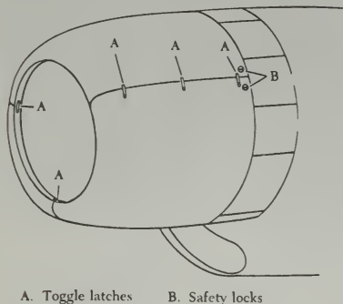
FIGURE 6-39. Ring cowl panel assembly.
